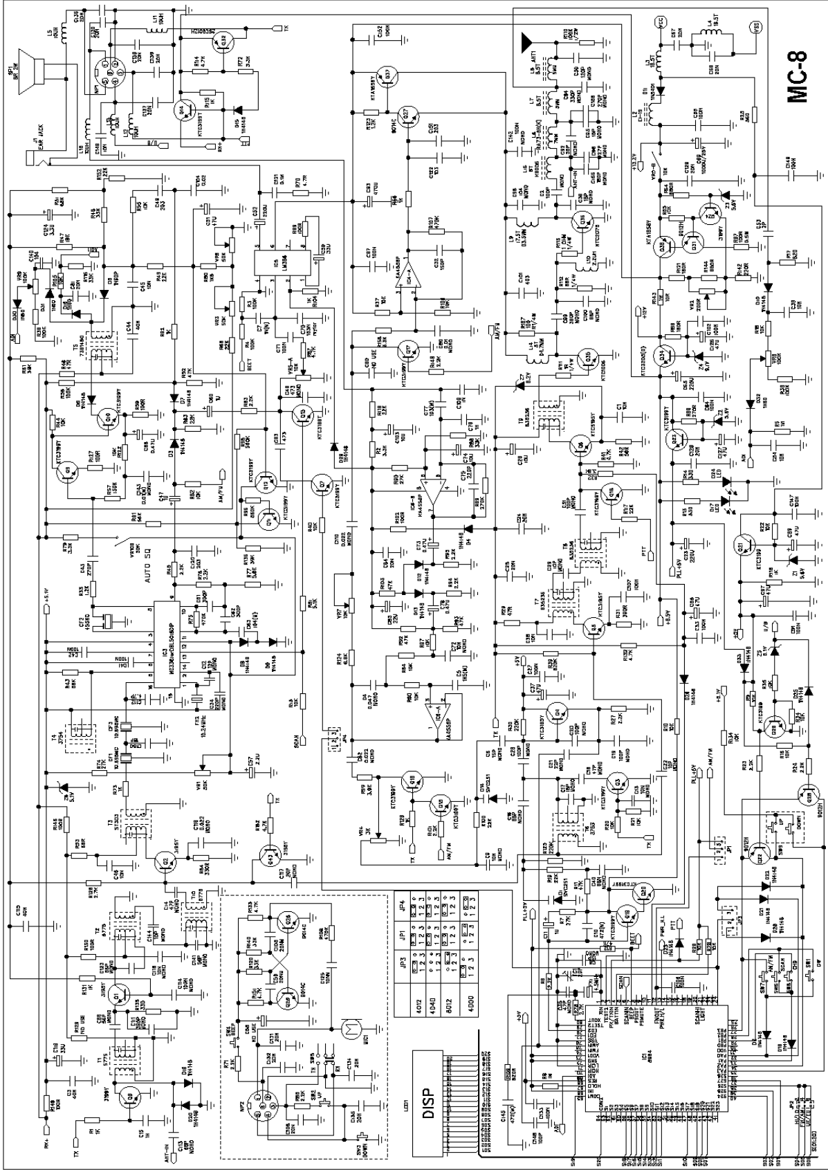
TEAM MC-8 Schaltplan / Schematic Diagram / Schema de principe / Schema elettrico
